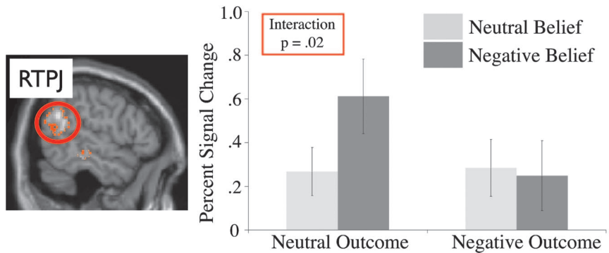
Fig. 3. PSC from rest in the RTPJ. (Left) Brain regions where the BOLD signal was higher for (nonmoral) stories about beliefs than (nonmoral) stories about physical representations ( n = 10 , random-effects analysis, P < 0.001 uncorrected). These data were used to define ROIs. (Right) The PSC in the RTPJ during the story segment when the protagonist's belief was stated ("Belief"). Error bars correspond to standard error.
